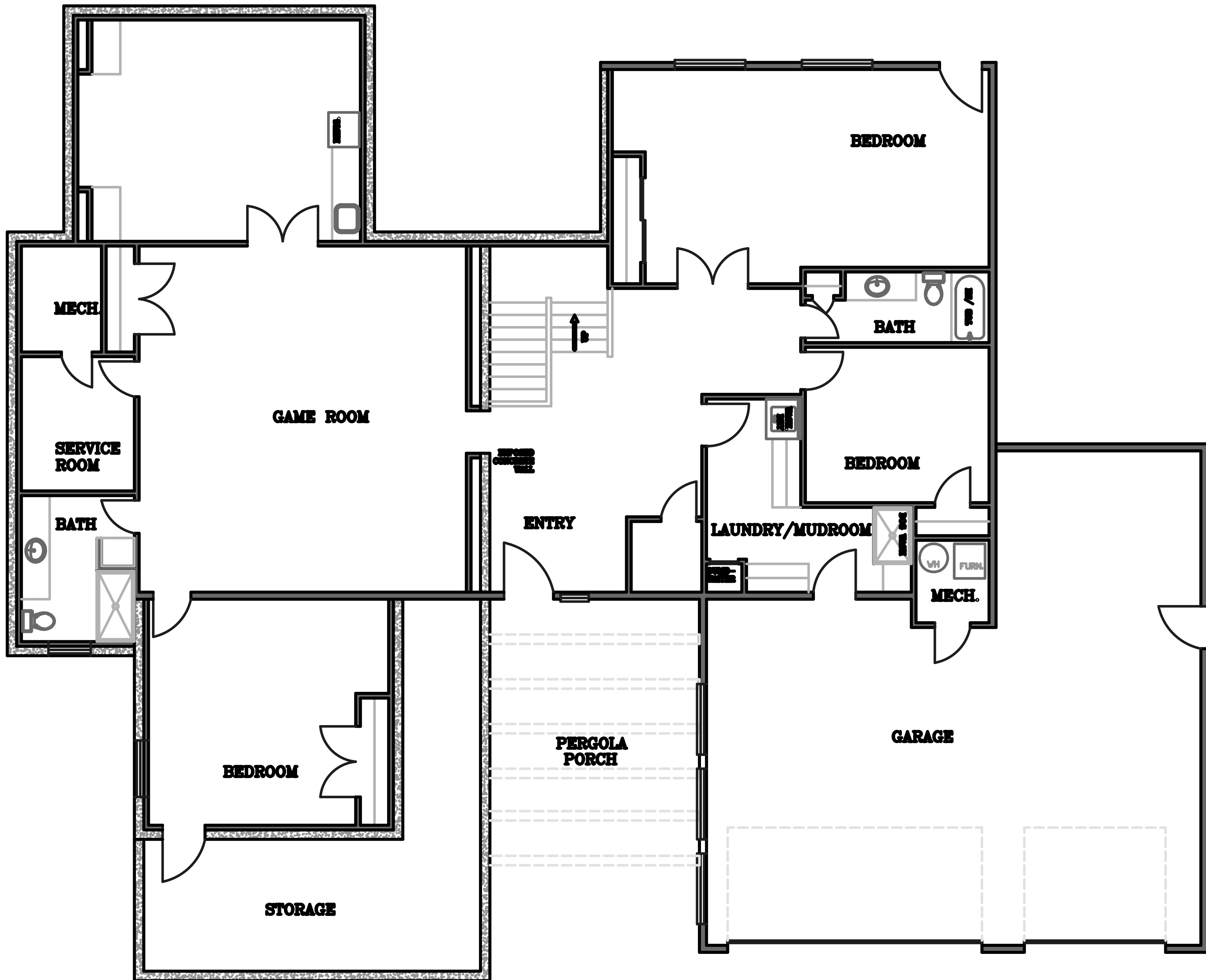
GROUND LEVEL
