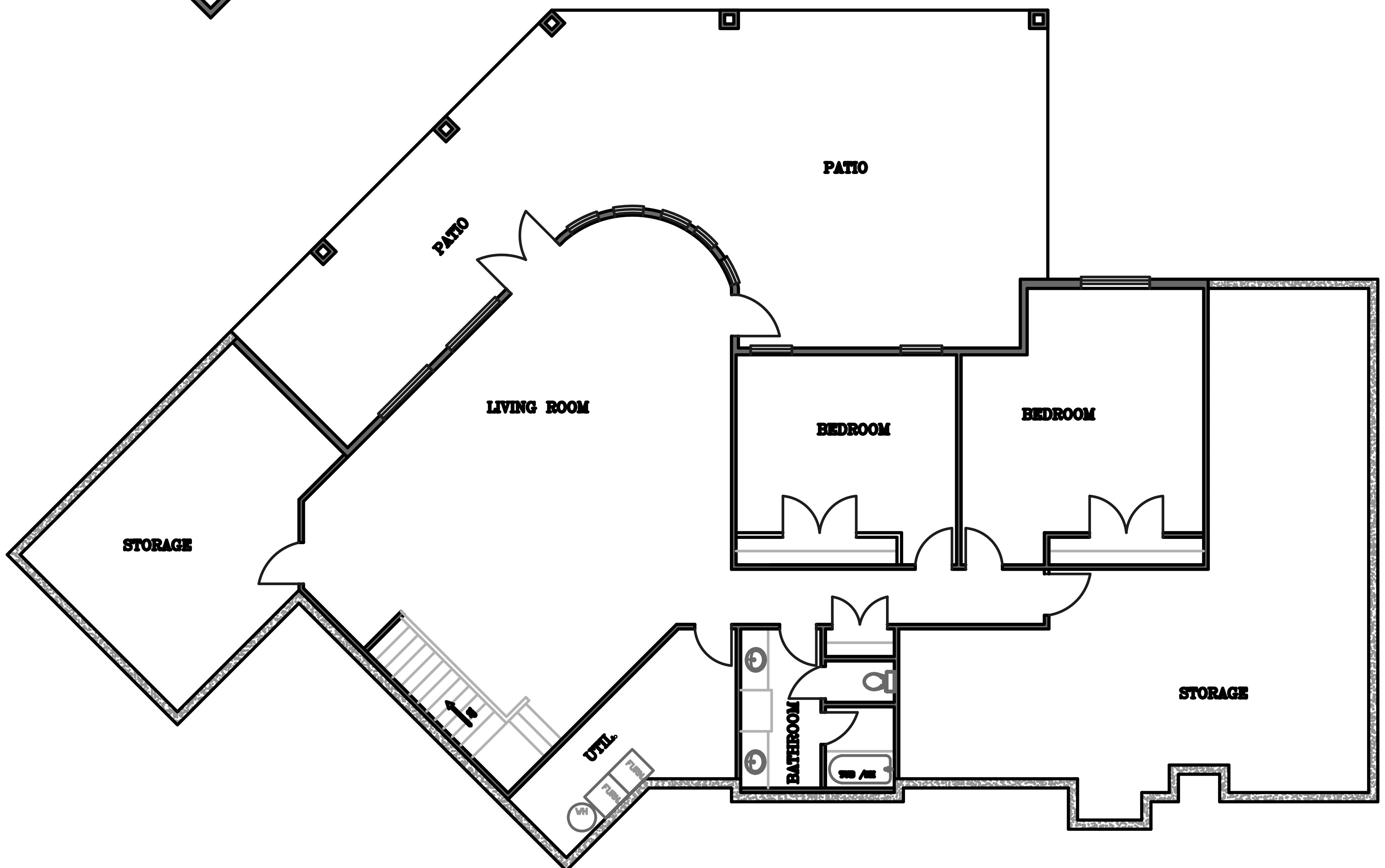
MILVERSTEAD RESIDENCE
